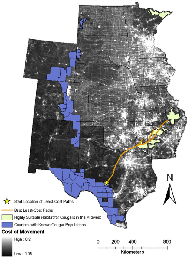
Fig. 2 – Best potential dispersal corridor from source area (i.e., easternmost areas in current western cougar ranges containing known breeding populations) to areas of highly suitable potential cougar habitat in midwestern North America.
