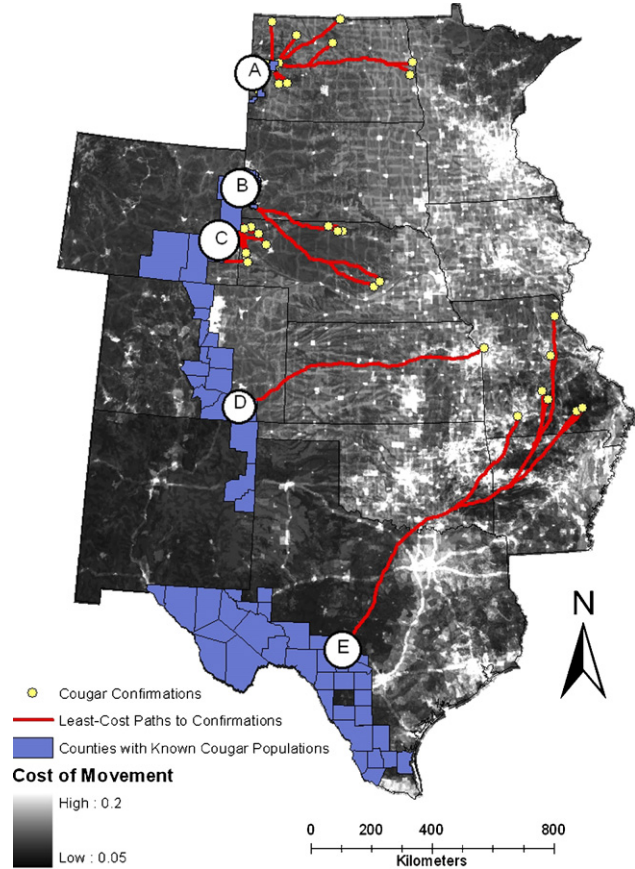
Fig. 3 – Potential cougar dispersal corridors from source area (i.e., easternmost areas in current western cougar ranges containing known breeding populations) to cougar confirmations in North Dakota, Nebraska, and Missouri. Starting points for least-cost paths were: A. Badlands, ND; B. Black Hills, SD; C. Platte and Niobrara Counties, WY; D. Las Animas County, CO; E. Kimble County, TX. Dates of confirmations range from 1990 to 2006 and confirmations are exact coordinate locations of cougars.
